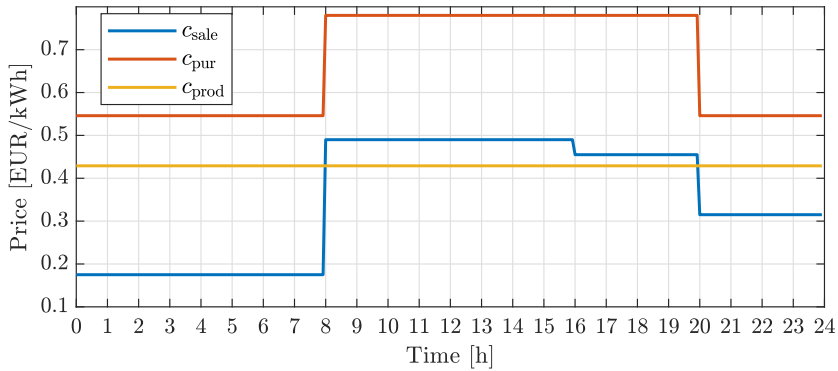
Figure 4.6: Electricity purchase ( c_{\text{pur}} ), sale ( c_{\text{sale}} ), and production ( c_{\text{prod}} ) prices in the considered simulation for the case study of Section 4.6.1 related to the control algorithm presented in Section 4.3.
